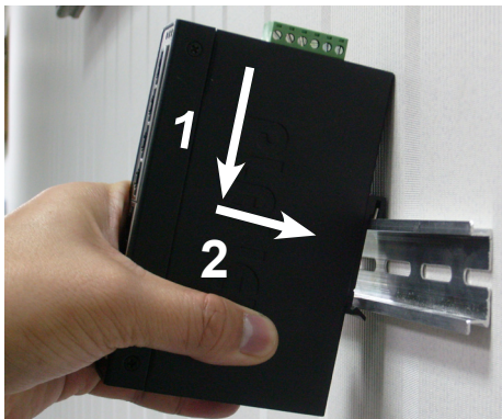
Figure 6: Install Industrial Equipment in DIN-Rail mount.
