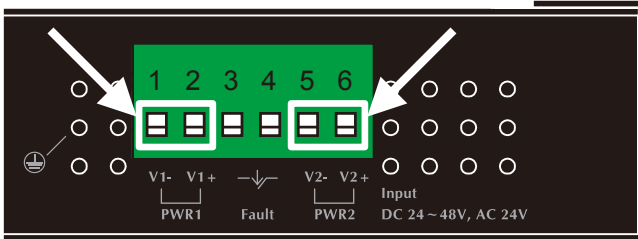
Figure 2: Power input PINs.
